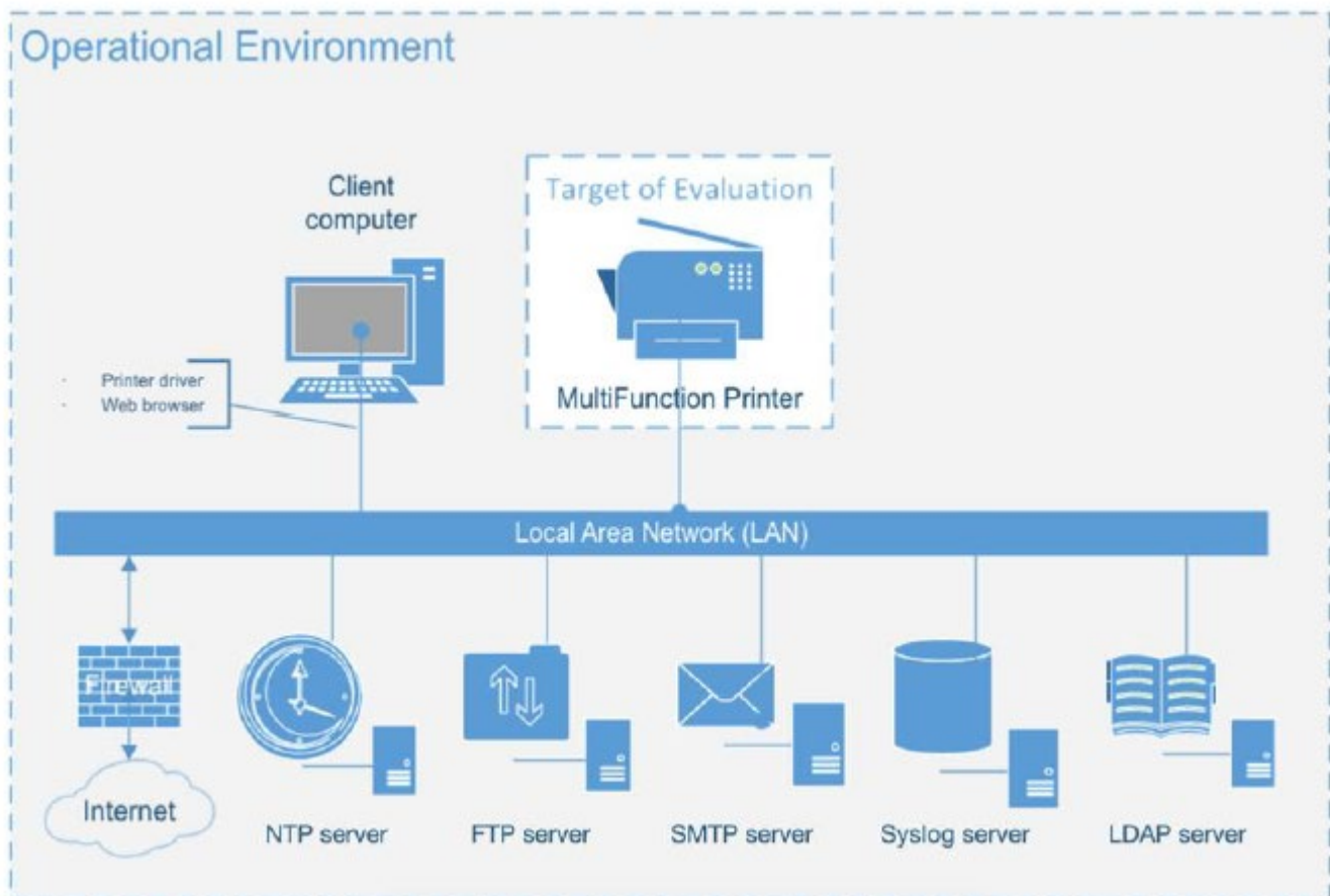
Figure 1: TOE Architecture
